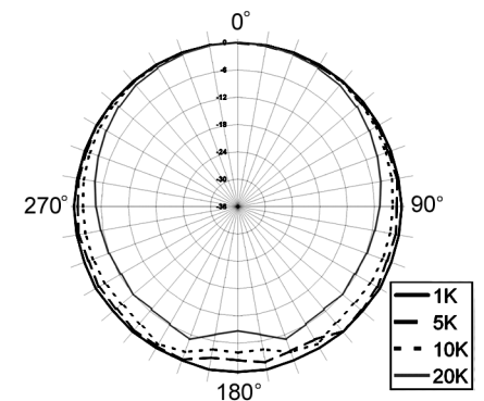
Fig 4. Polar Response (Typical) of QTC30
