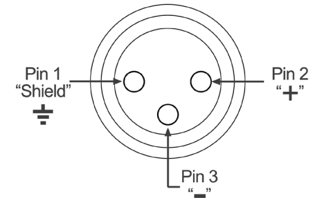
Fig 1. XLR Output Connector Assignment of QTC30
