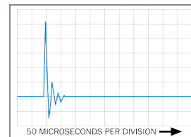
Impulse Response
