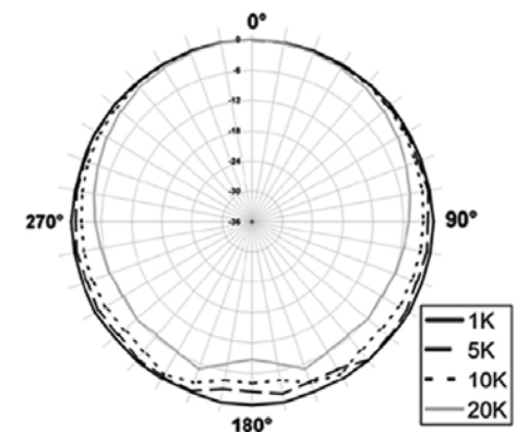
Fig 3. Polar Response (Typical) of M50, 1dB/div.
