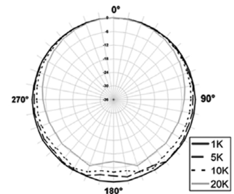
Fig 3. Polar Response (Typical) of M23, 1dB/div.
